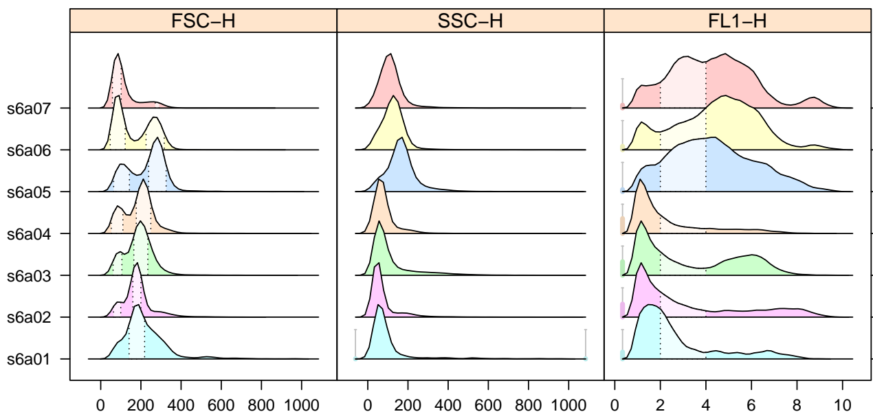
Figure 8: Multiple densityplots with combination of rectangleGate and curv2Filter .
