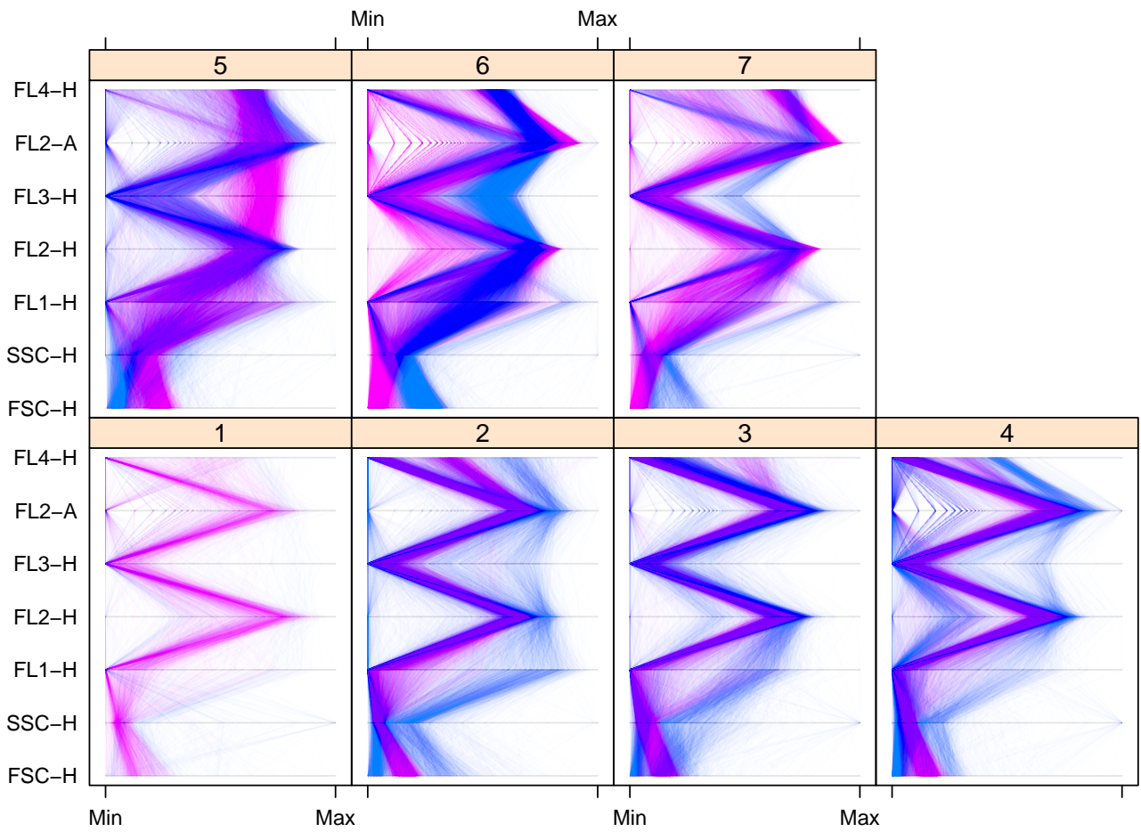
Figure 13: Parallel coordinates plot all channels excluding time.
