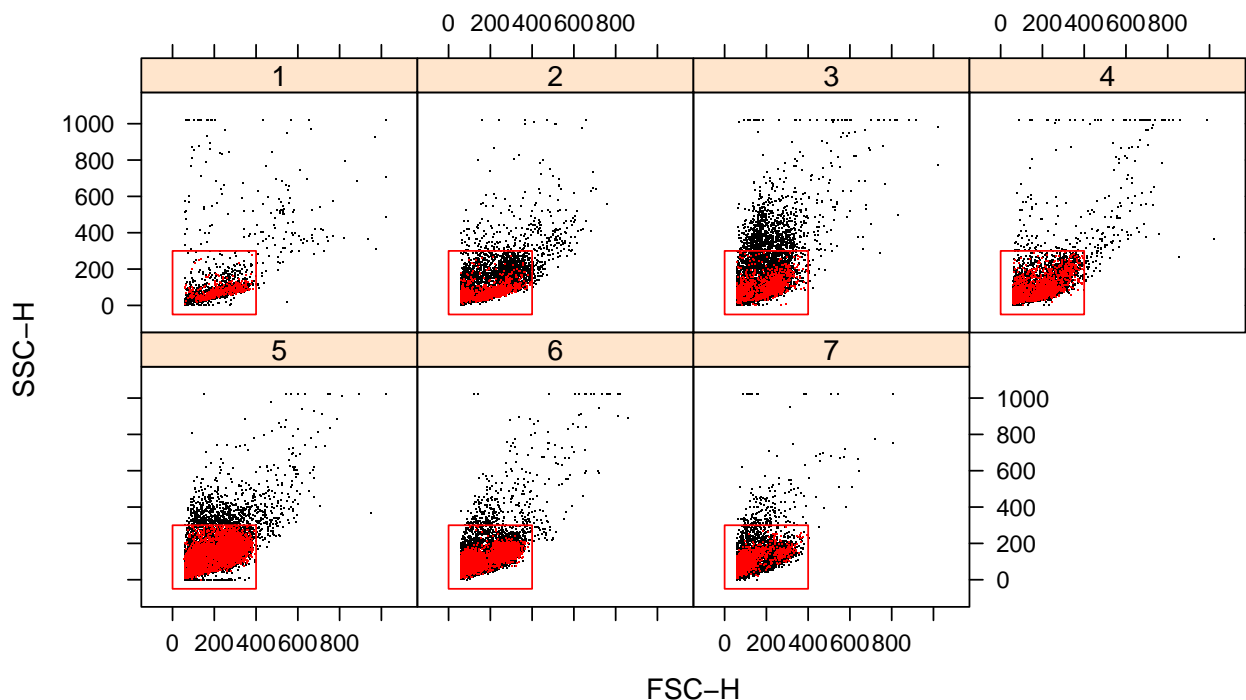
Figure 4: Three-dimensional rectangle gate with outline in the FSC-H-FL4-H non-smooth xyplot.
