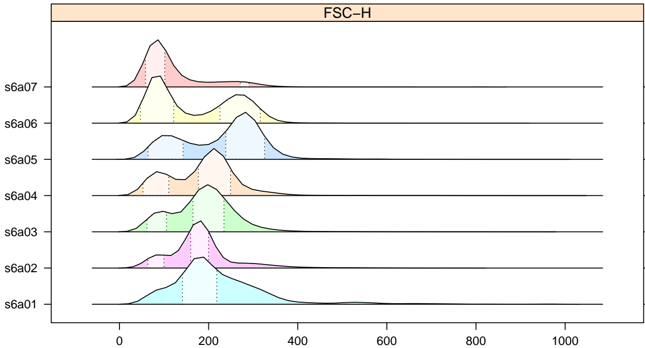
Figure 7: High density areas identified by curv1Filter .
