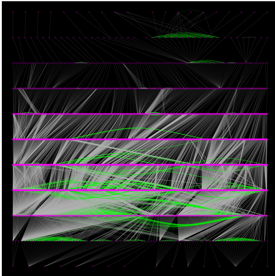
Figure 4: Multiroot-tree (hierarchical) layout style of artificial network 1 ( |V| = 10,000 , |E| = 32,761 )
