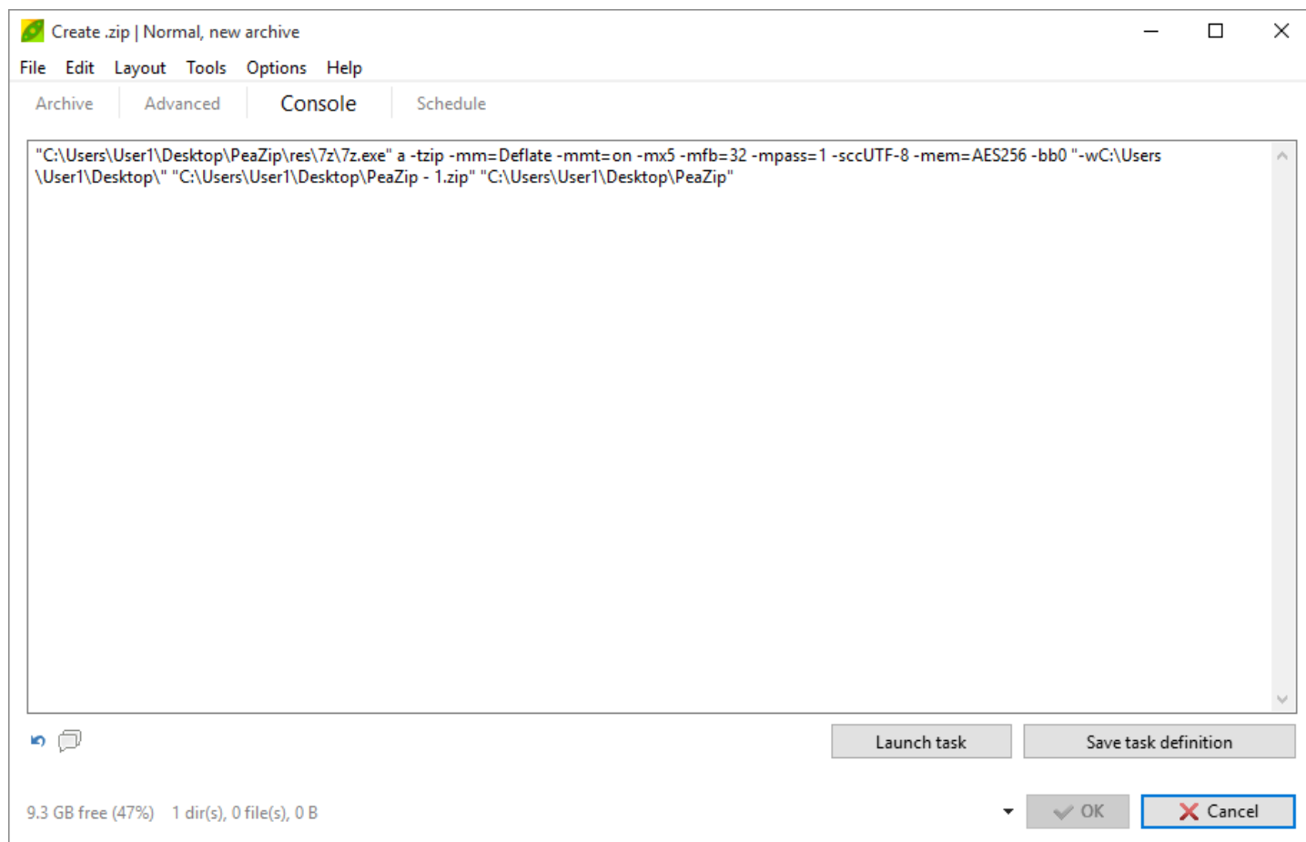
Image 17: Console tab
