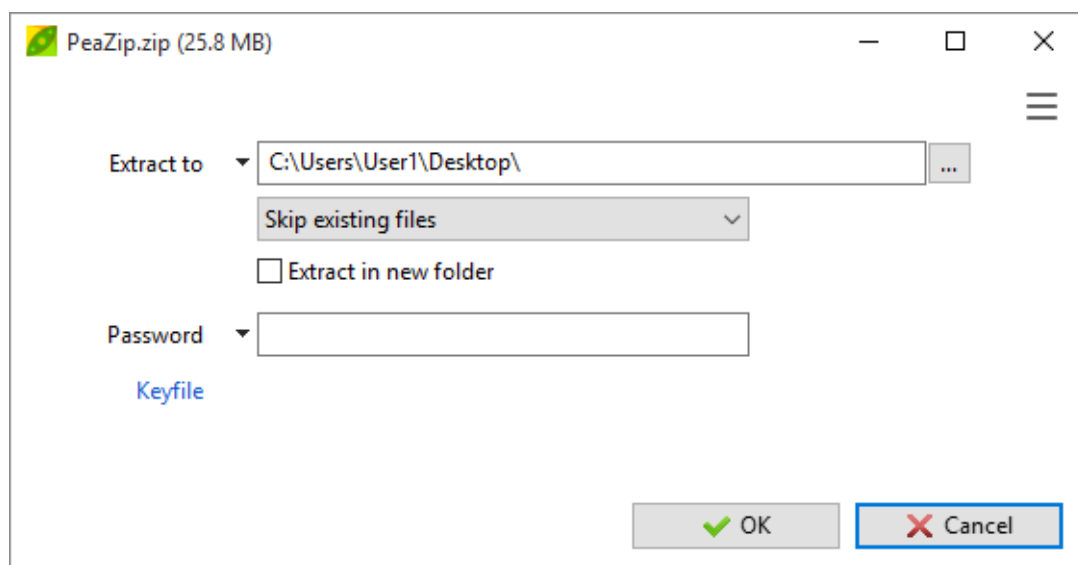
Image 21: PeaExtractor
