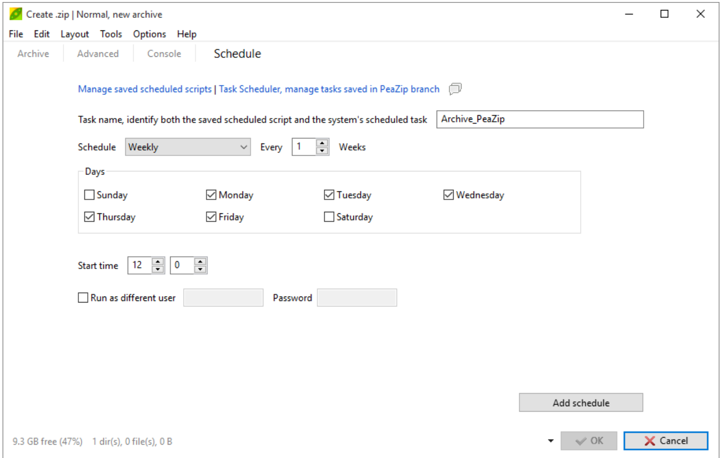
Image 18: Schedule tab
