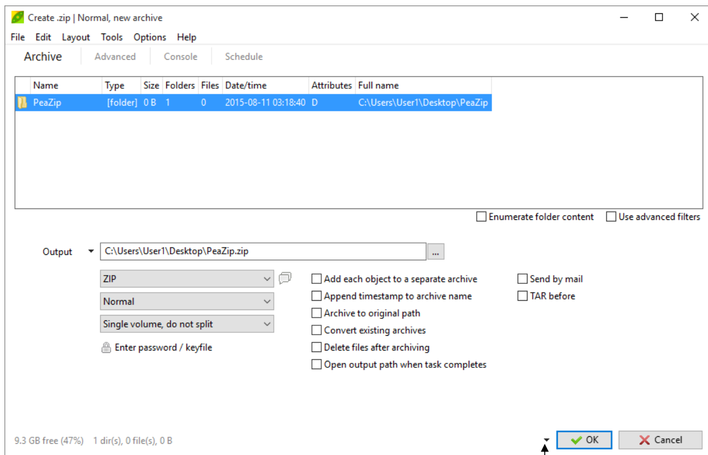
Compression profiles and Favourite formats context menu
