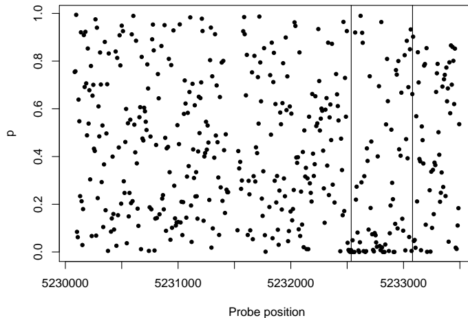
Figure 1: Probe-level p-values
