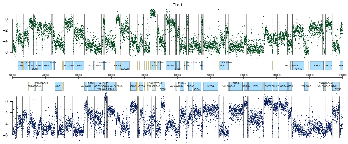
Figure 4: Along-chromosome plot similar to Figure 1 of [1].
